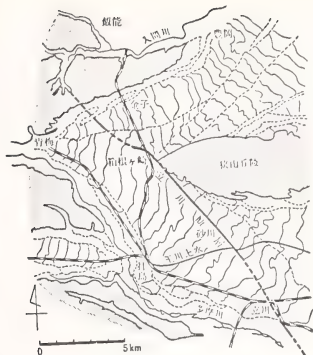
Fig. 4 Tachikawa fault
